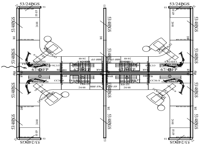
2D PLAN LAYOUT
