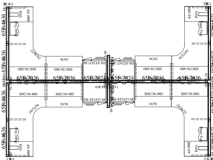
2D PLAN LAYOUT
